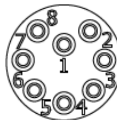
Male Pins Face View
